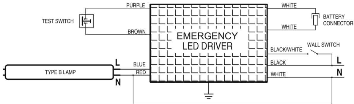
SINGLE-END INSTALLATION
