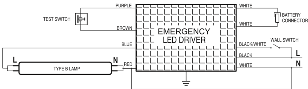
DOUBLE-END INSTALLATION
