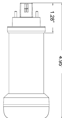
G24d-2 base, 2-pin
