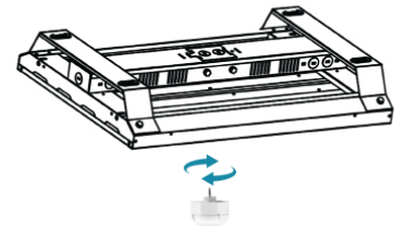
12VDC Microwave Sensor Order Code: 11795 Note: One remote control (11796) for multiple microwave sensors.
